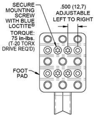
FOOT PAD DETAIL
